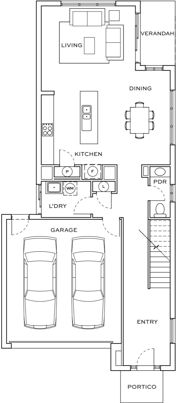
GROUND FLOOR
