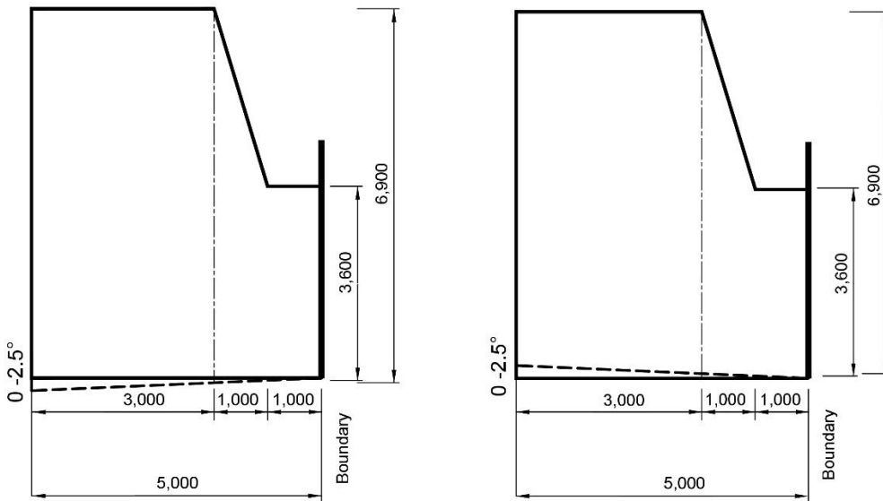
Typical Side and Rear Boundary for lots marked with *
